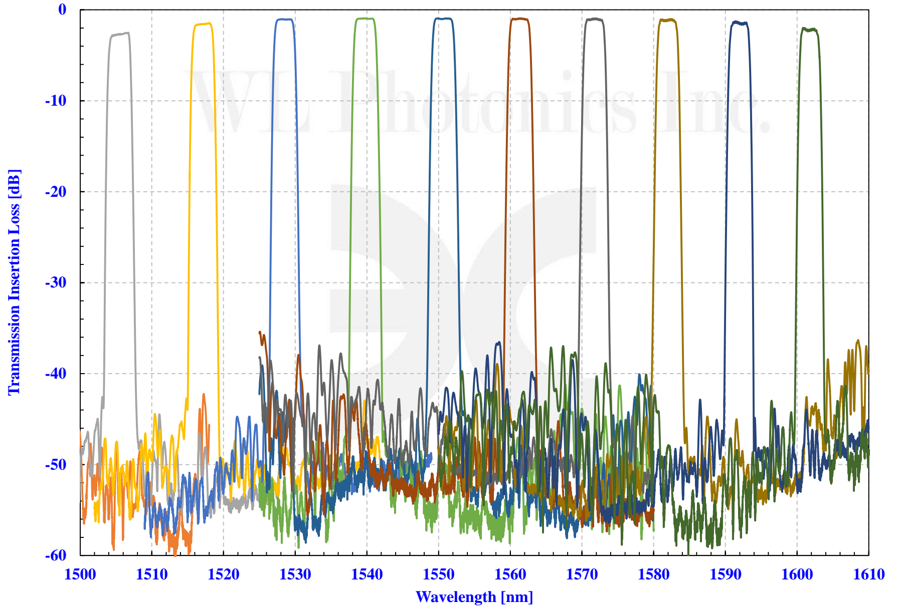
Transmission Spectrum of 3.0 nm Flat-Top P-Grade Tunable Filter over C-Band
