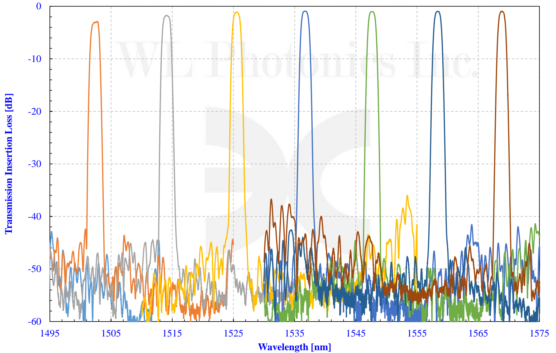
Transmission Spectrum of 1.25nm Flat-Top P- Grade Tunable Filter over C Band
