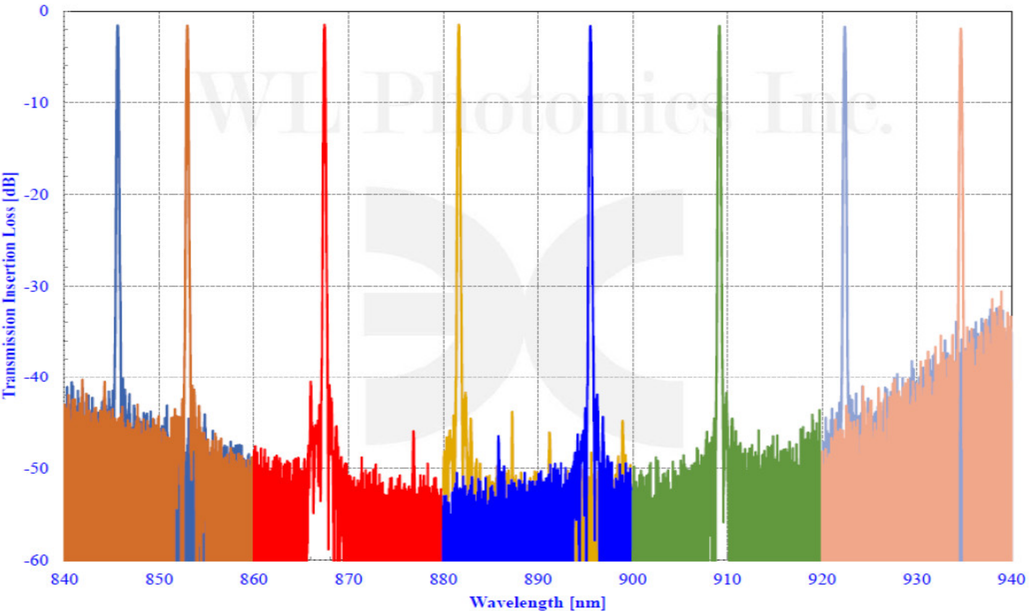
Transmission Spectra of 0.15nm Tunable Optical Filter over 830-950nm
