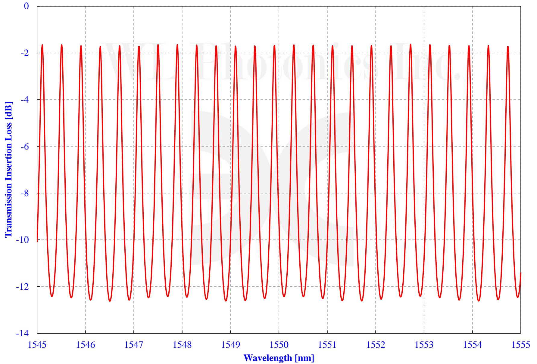
Typical Transmission of 50GHz Fiber-Pigtailed Etalon over C-Band
