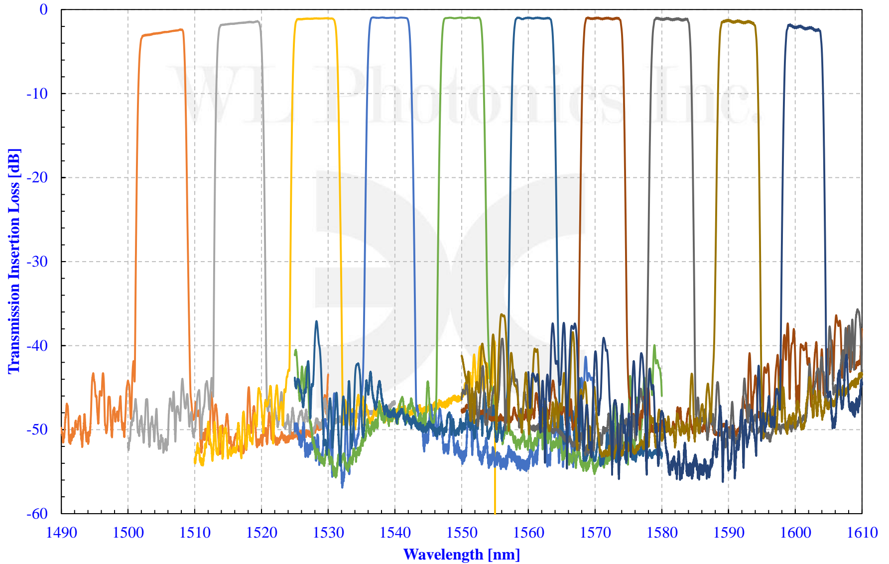
Transmission Spectrum of 6.0 nm Flat-Top P-Grade Tunable Filter over C -Band
