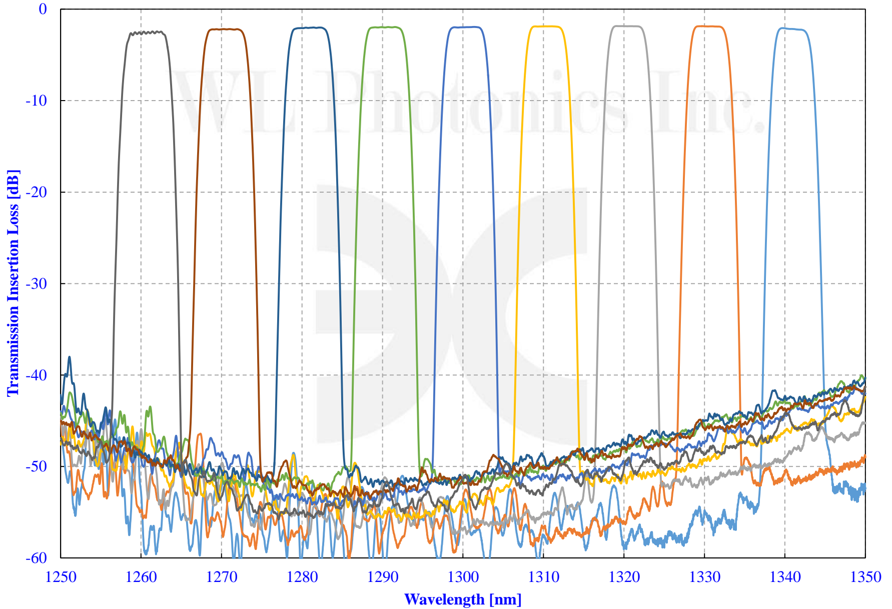
Transmission Spectrum of 5.0nm Flat-Top Tunable Filter over 1260-1340nm
