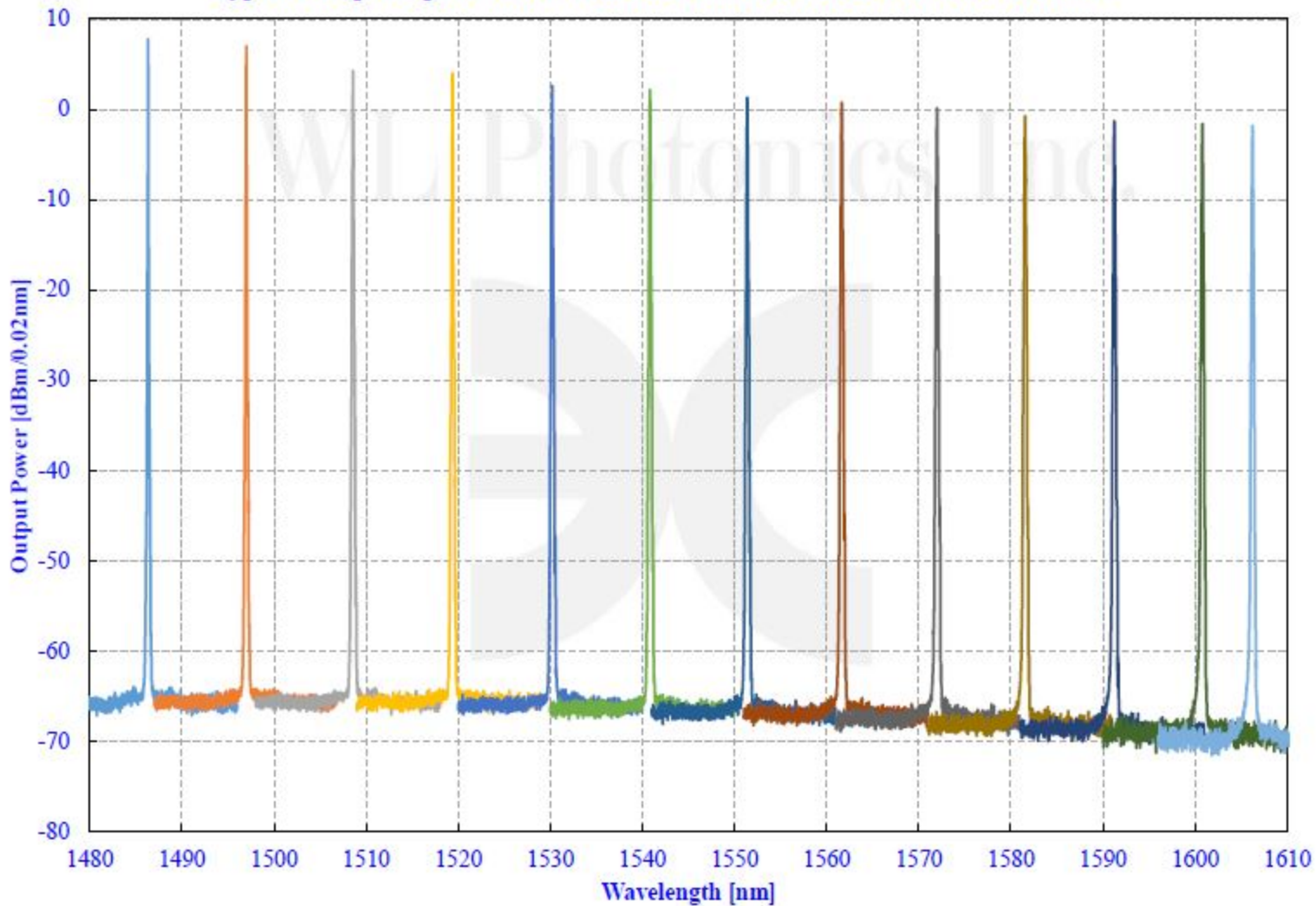
Typical Output Spectrum of Tunable Fiber Laser over over 1460-1610nm
