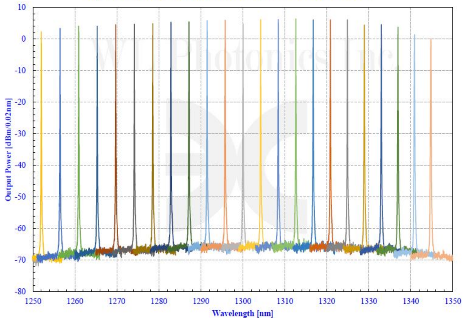
Typical Output Spectrum of Tunable Fiber Laser over 1250-1350 nm
