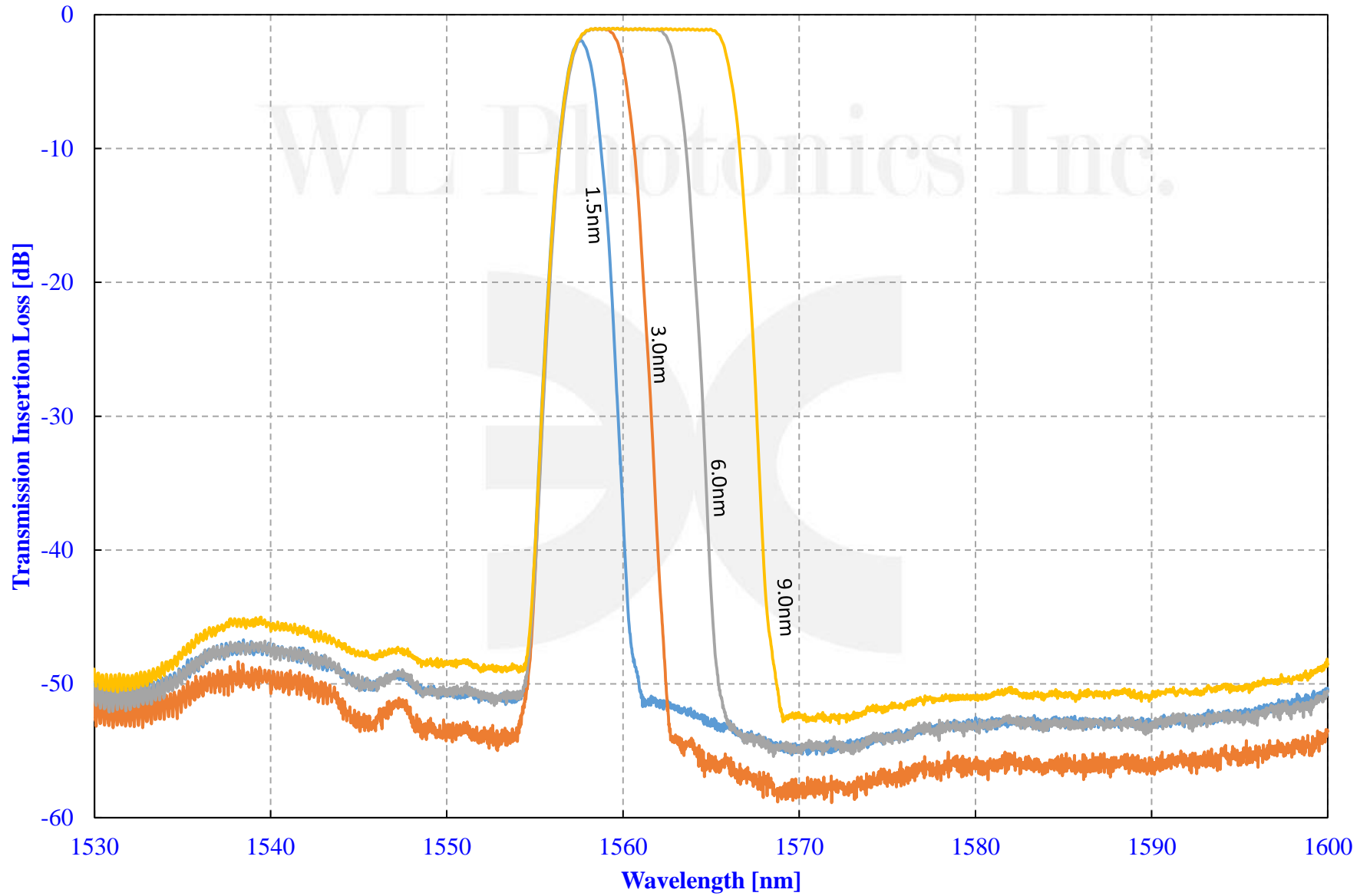
Transmission Spectrum of Bandwidth Adjustment over C-Band (Standard Version)
