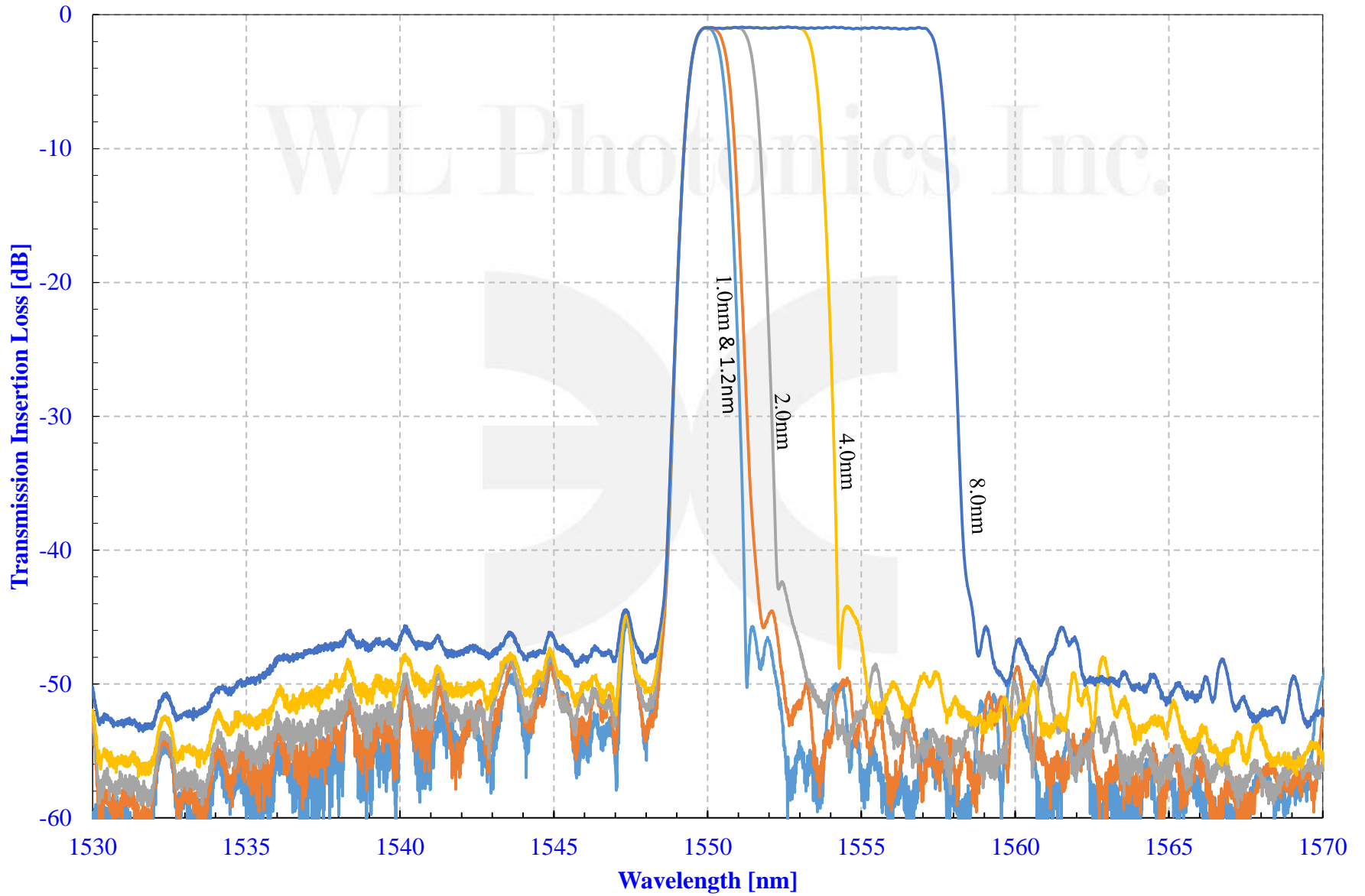
Transmission Spectrum of Bandwidth Adjustment over C-Band (Premium Version)
